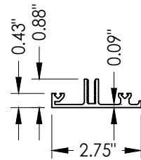
D HORIZONTAL MEMBER
