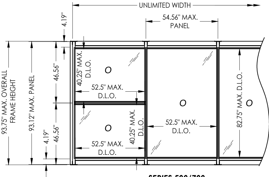
SERIES 500/700 Multi-span
