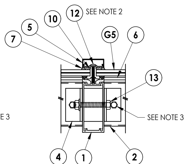
2 CROSS SECTION
