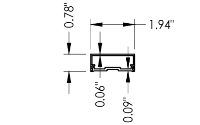
B COMPRESSION PLATE & COVER
