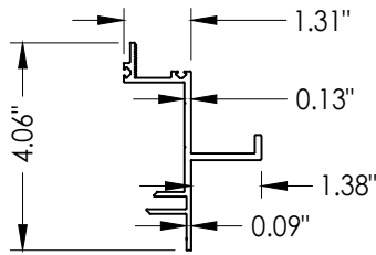
H ALUM. FRAME MEMBER
