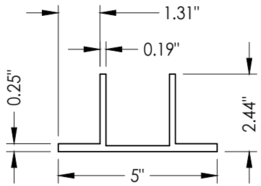
G BRAC-1 SADDLE CLIP 2" wide
