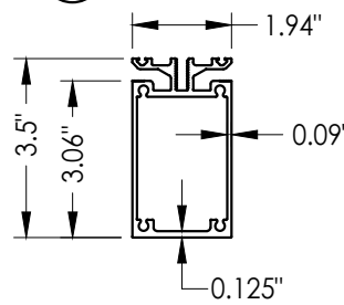
1 SERIES 350 RAFTER
