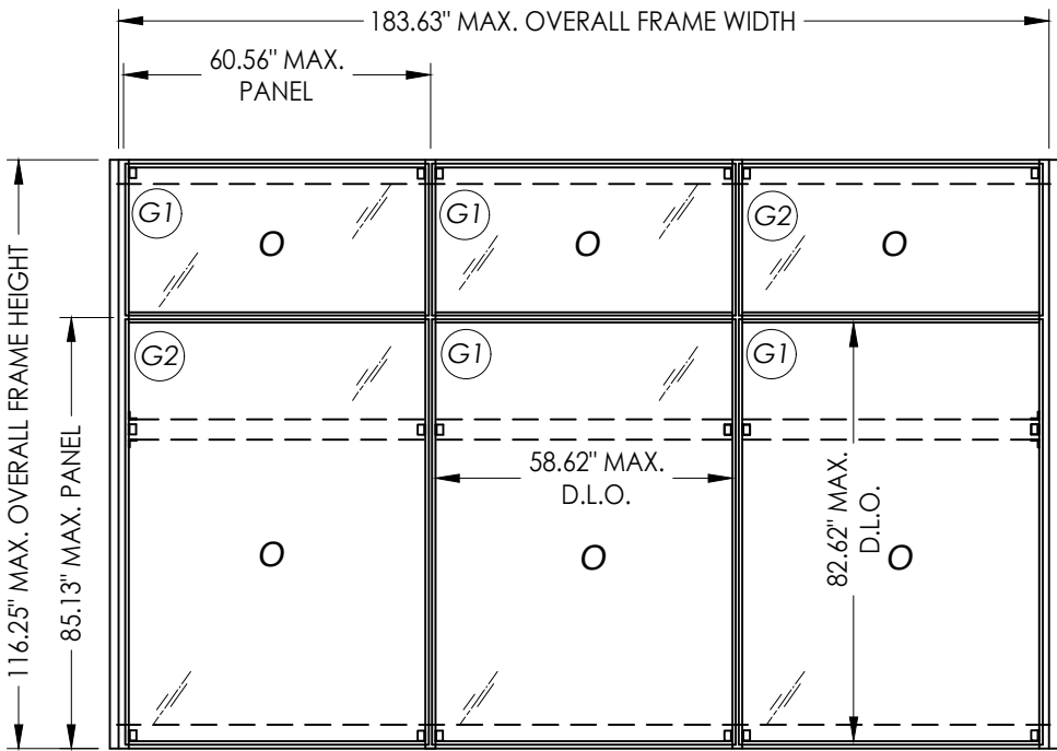
SERIES 350/500/700 Multi-span
