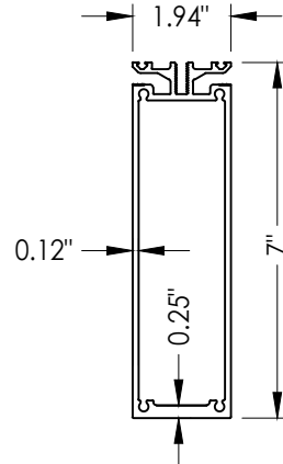
1 SERIES 700 RAFTER Optional
