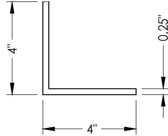
J ALUMINUM ANGLE CLIP 3.5" wide
