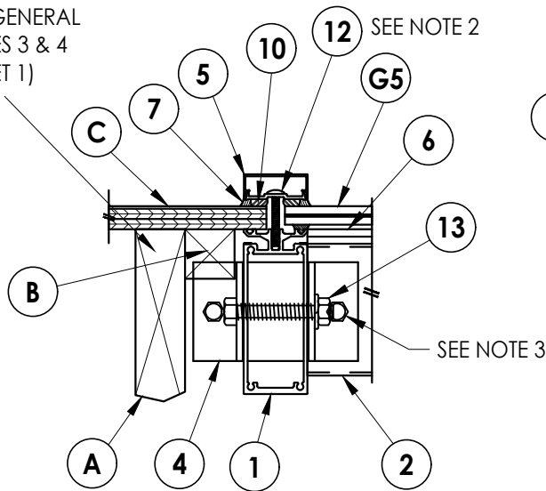
1 CROSS SECTION
